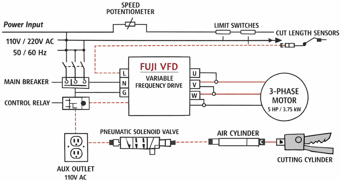
MOE / M4-10 REBAR CUTTER ELECTRICAL SCHEMATIC
